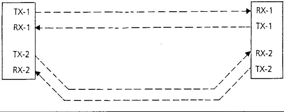
Figure 9. Two-terminal line, dual-channel with diverse channel routing
