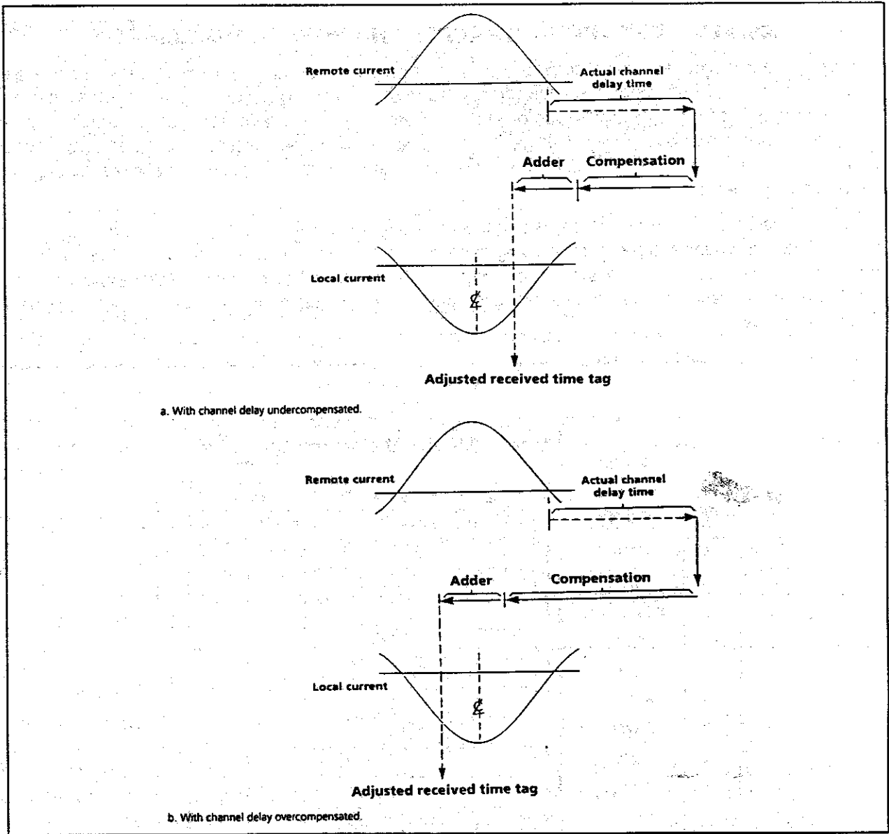
Figure 5. DML measurement
