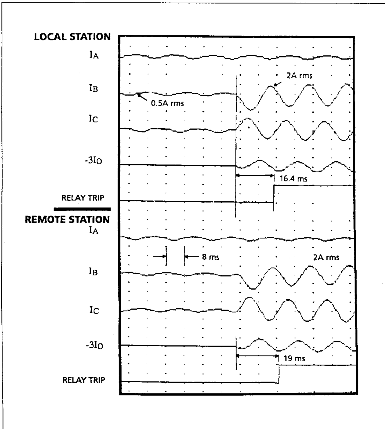
Figure 17. Internal double-line to ground (BC-G) fault
