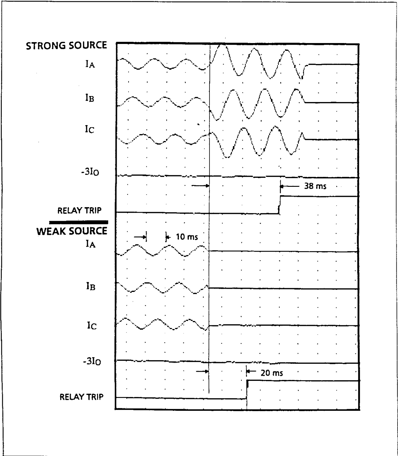
Figure 15. Weak-feed trip, 7.2-Kbps communication channel
