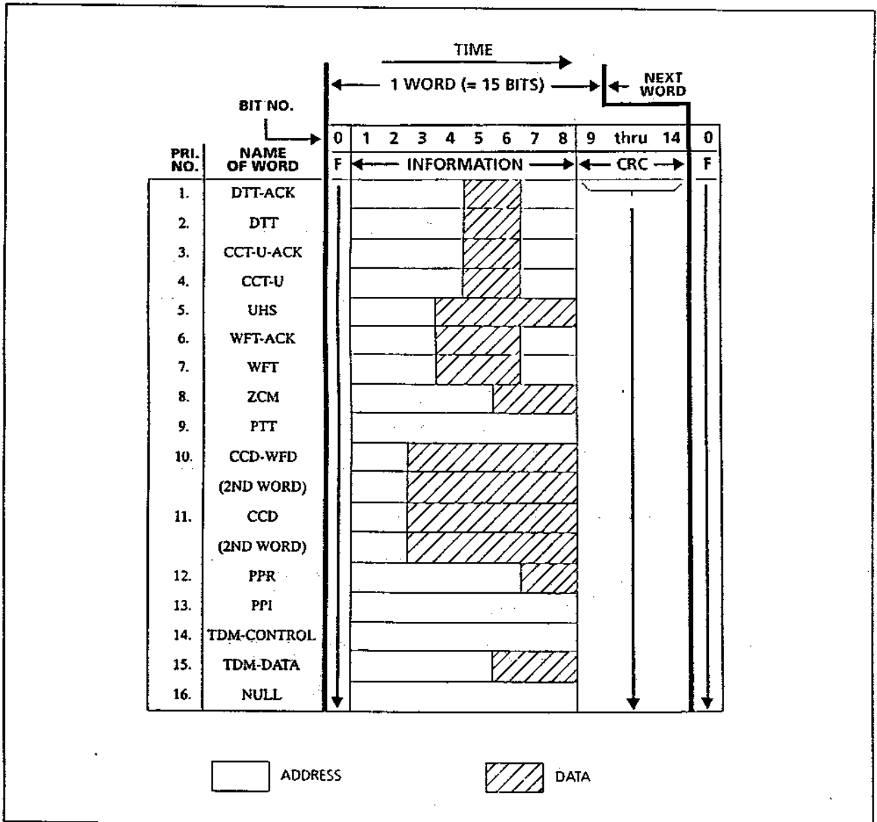
Figure 7. Charge comparison communications message structure
