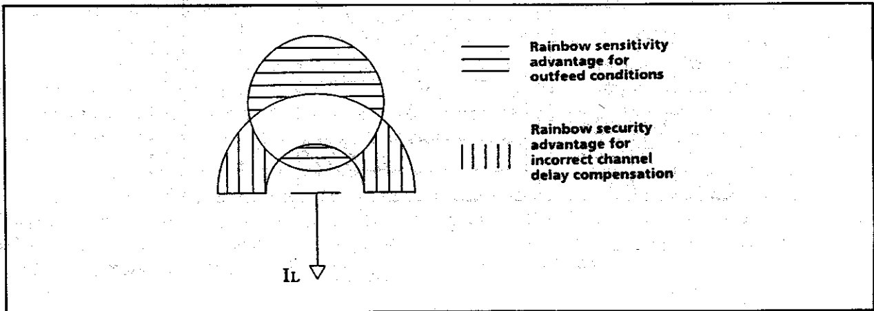
Figure 6. Rainbow characteristic vs. conventional circle characteristic
